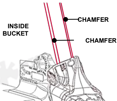
CHEEK DIMENSIONS
